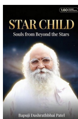
Star Child
